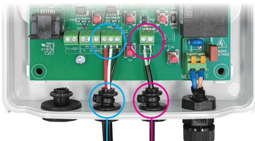
Figure 5. Modbus Connection
